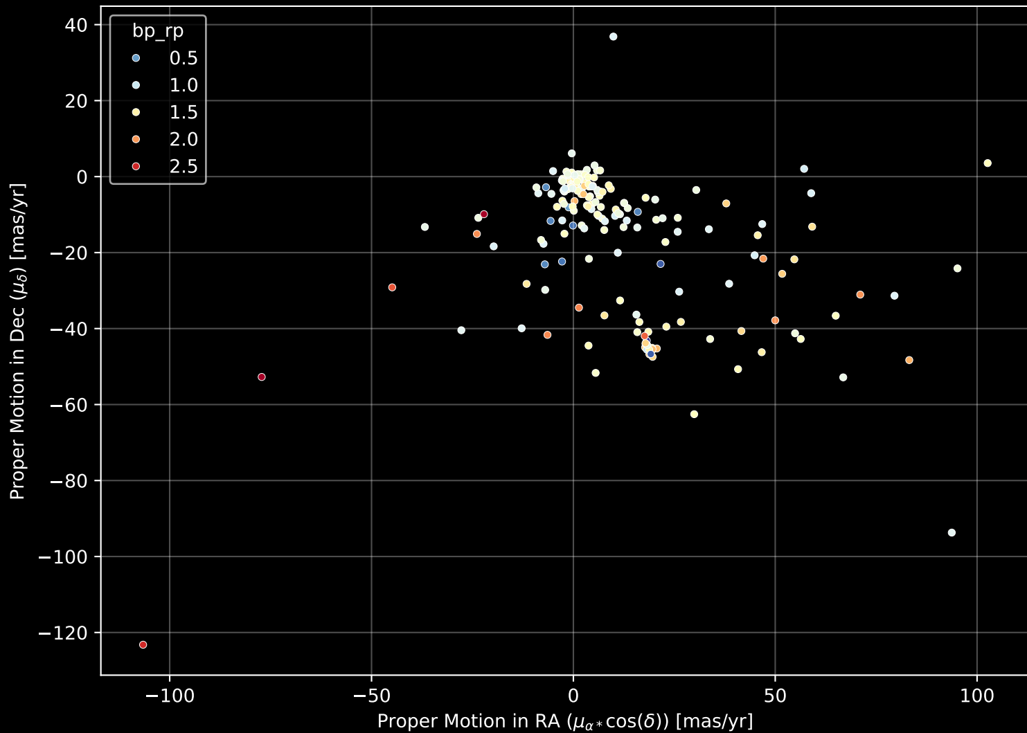
APOGEE DR17 Field: [K2_C4_168-21_btx] Proper Motion Diagram (n= 193)
