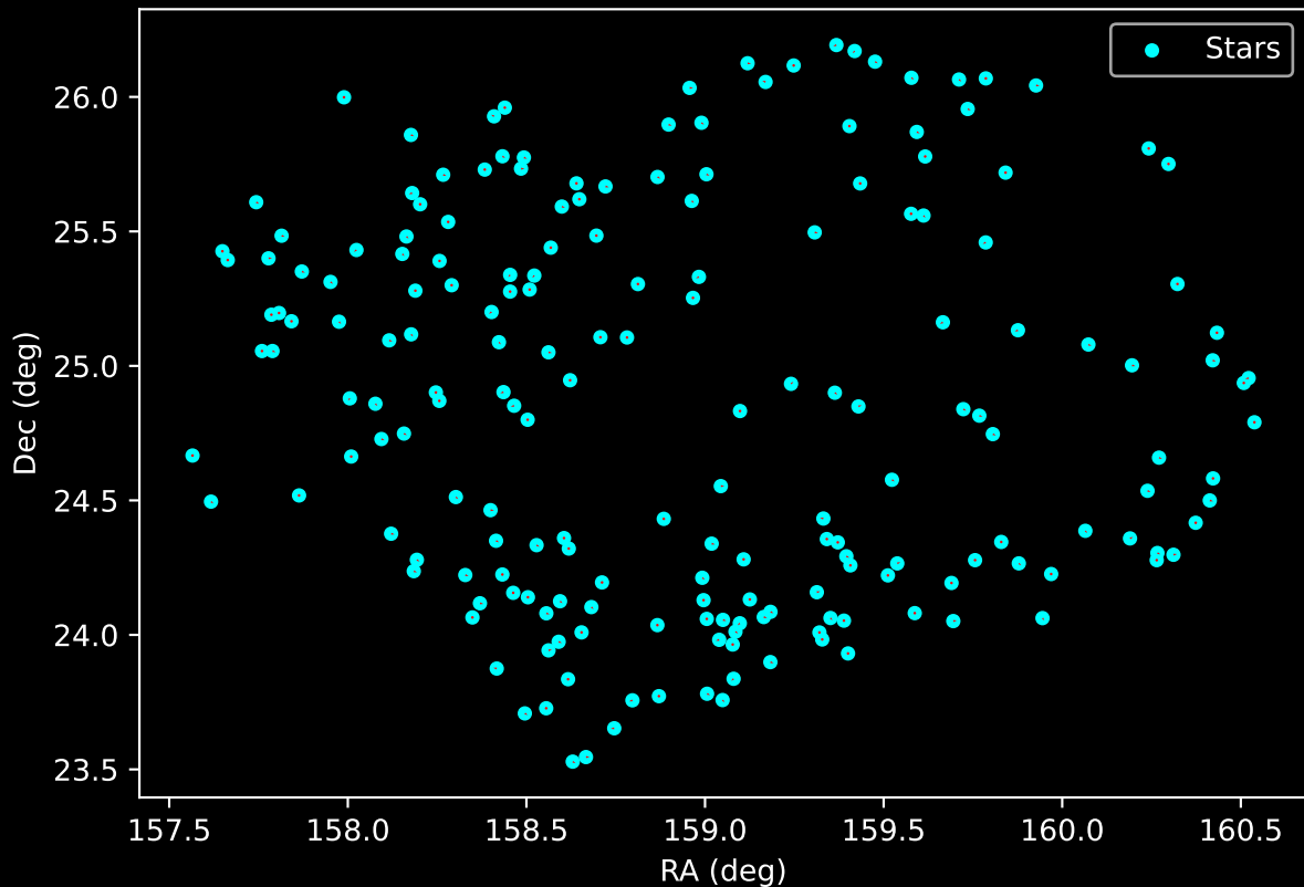
APOGEE DR17 Field: [K2_C4_168-21_btx] Proper Motion Vectors for Gaia Star Field (n= 193)
