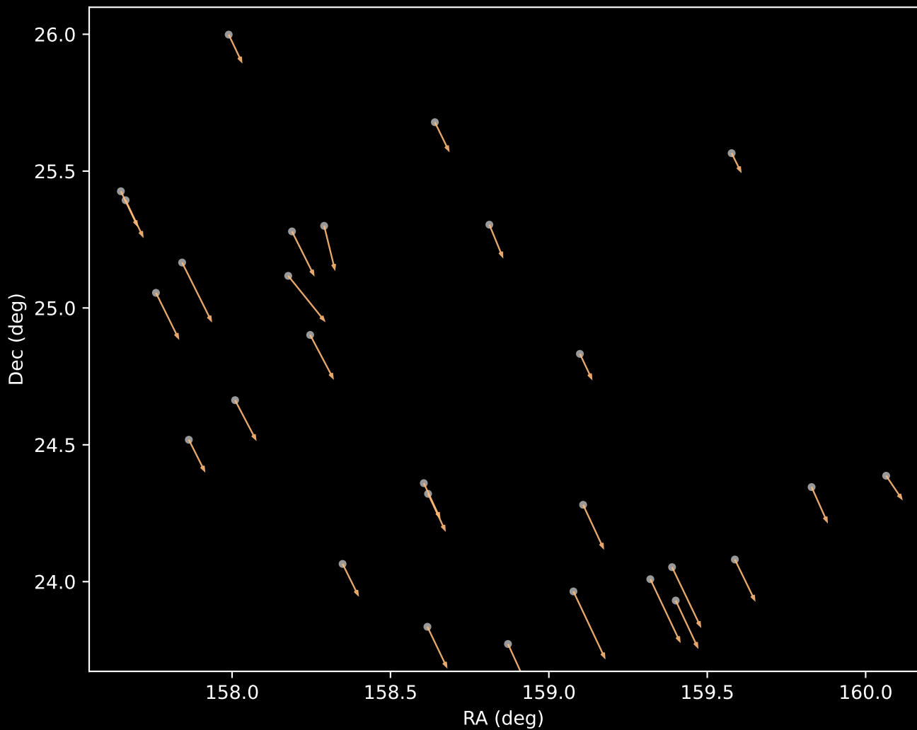
APOGEE DR17 Cluster 3 Proper Motion Vectors (n=28)
