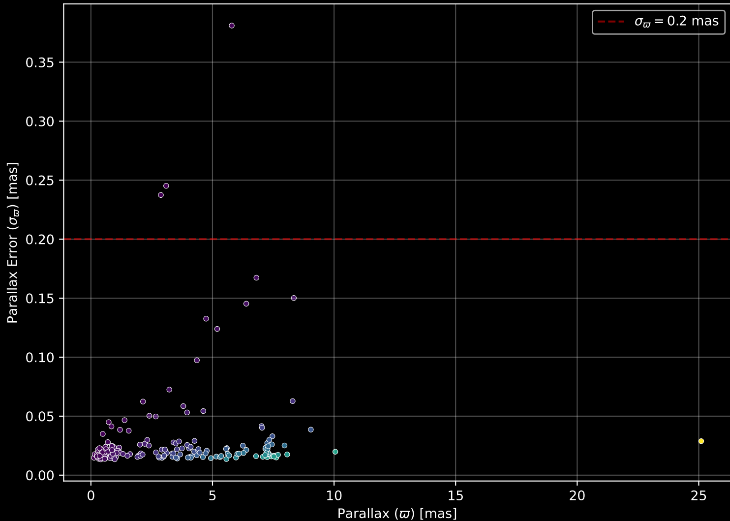
APOGEE DR17 Field: [K2_C4_168-21_btx] Parallax Quality (n= 193)
