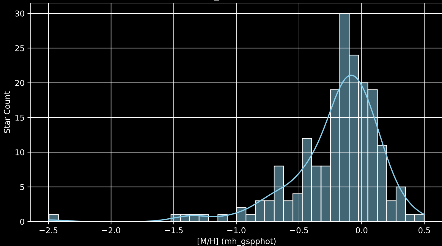
APOGEE DR17 Field: [K2_C4_168-21_btx [M/H] (mh_gspphot) (n= 191)
