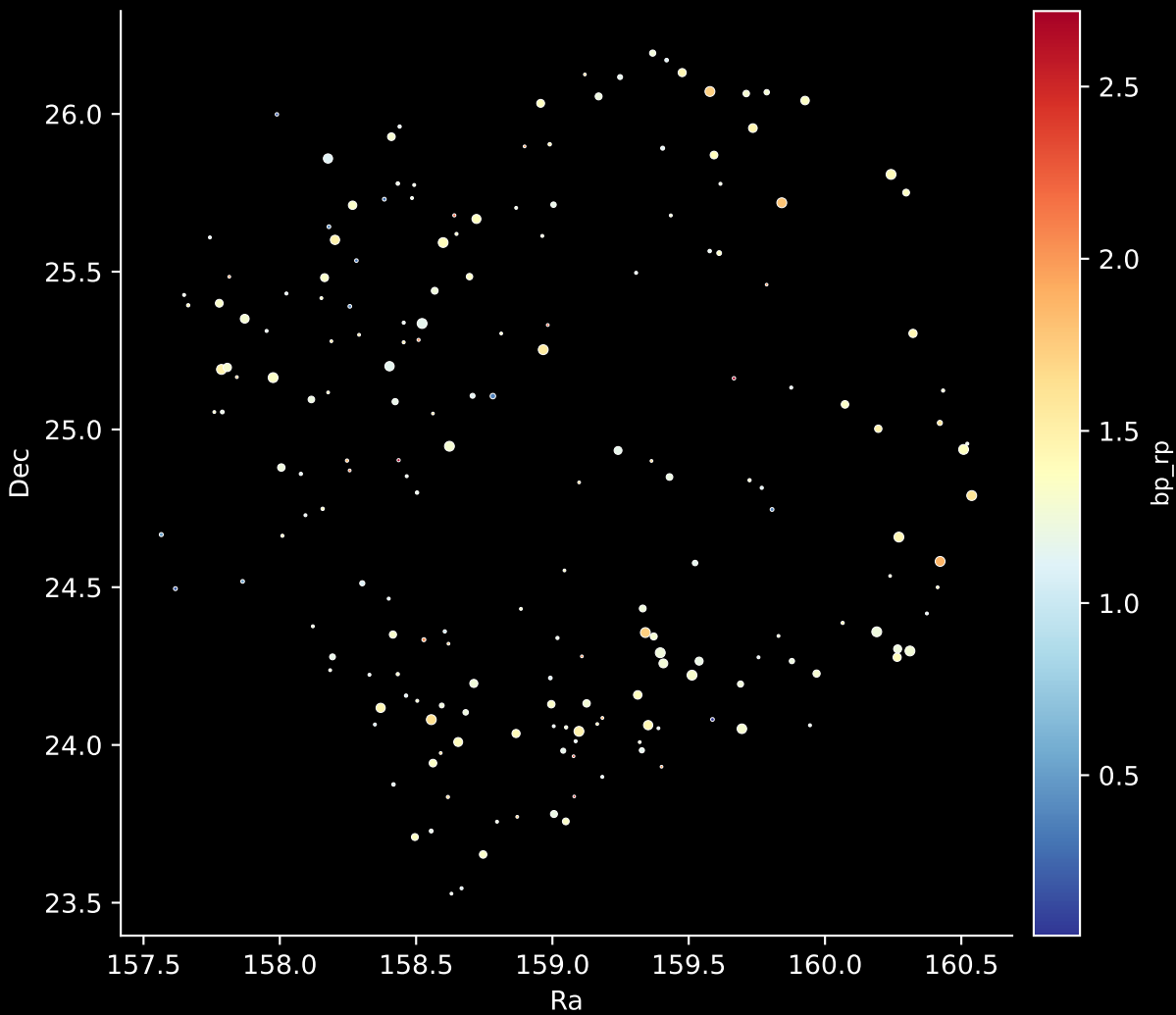
APOGEE DR17 Field: [K2_C4_168-21_btx] Stars: 193
