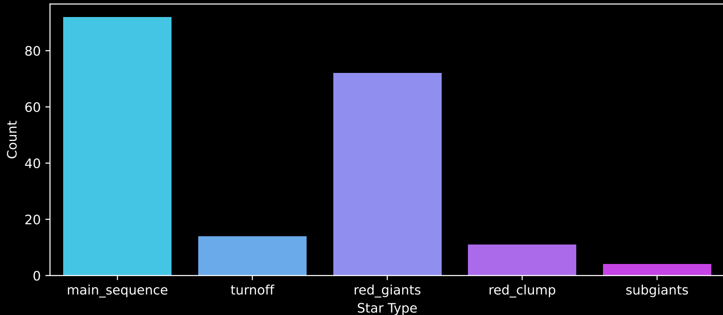
APOGEE DR17 Field: [K2_C4_168-21_btx] Count plot of Star Type
