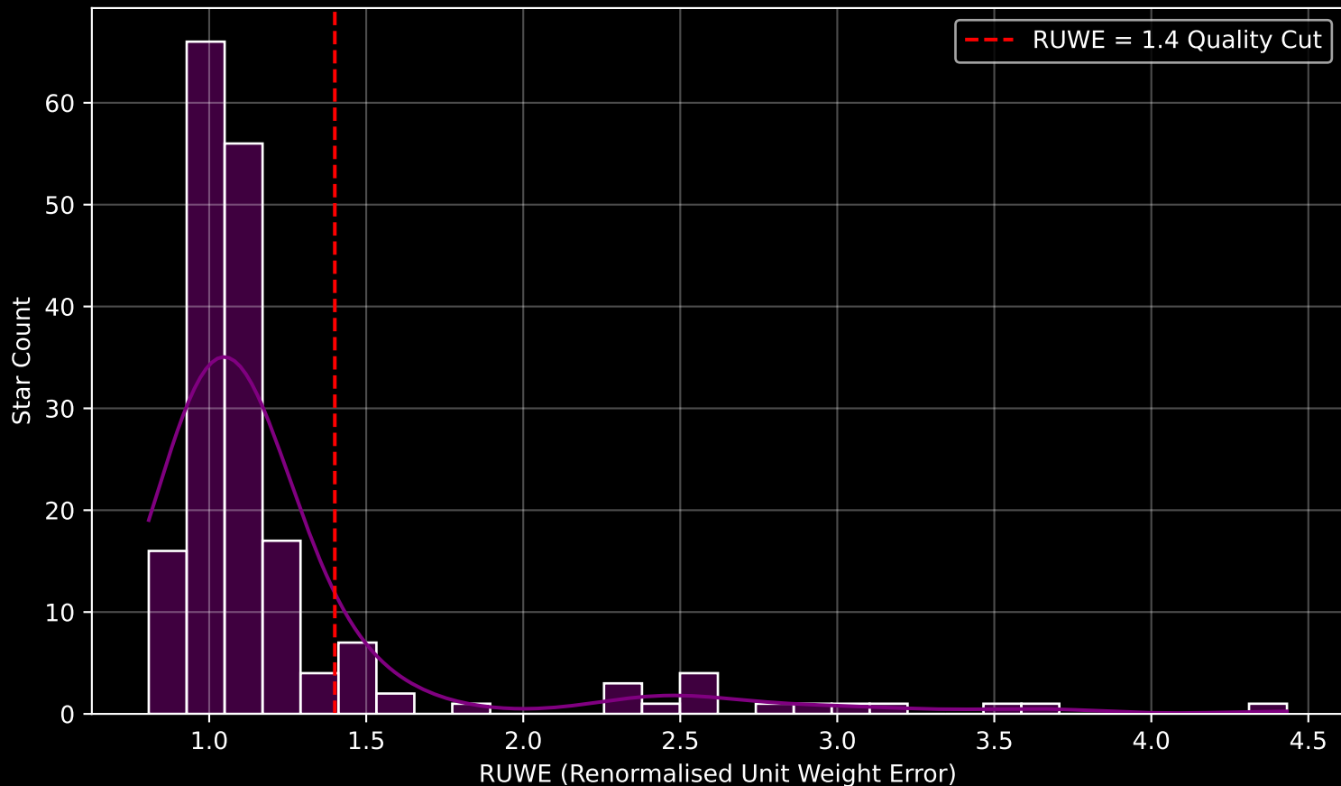
GAPOGEE DR17 Field [K2_C4_168-21_btx] RUWE Distribution (n= 184)
