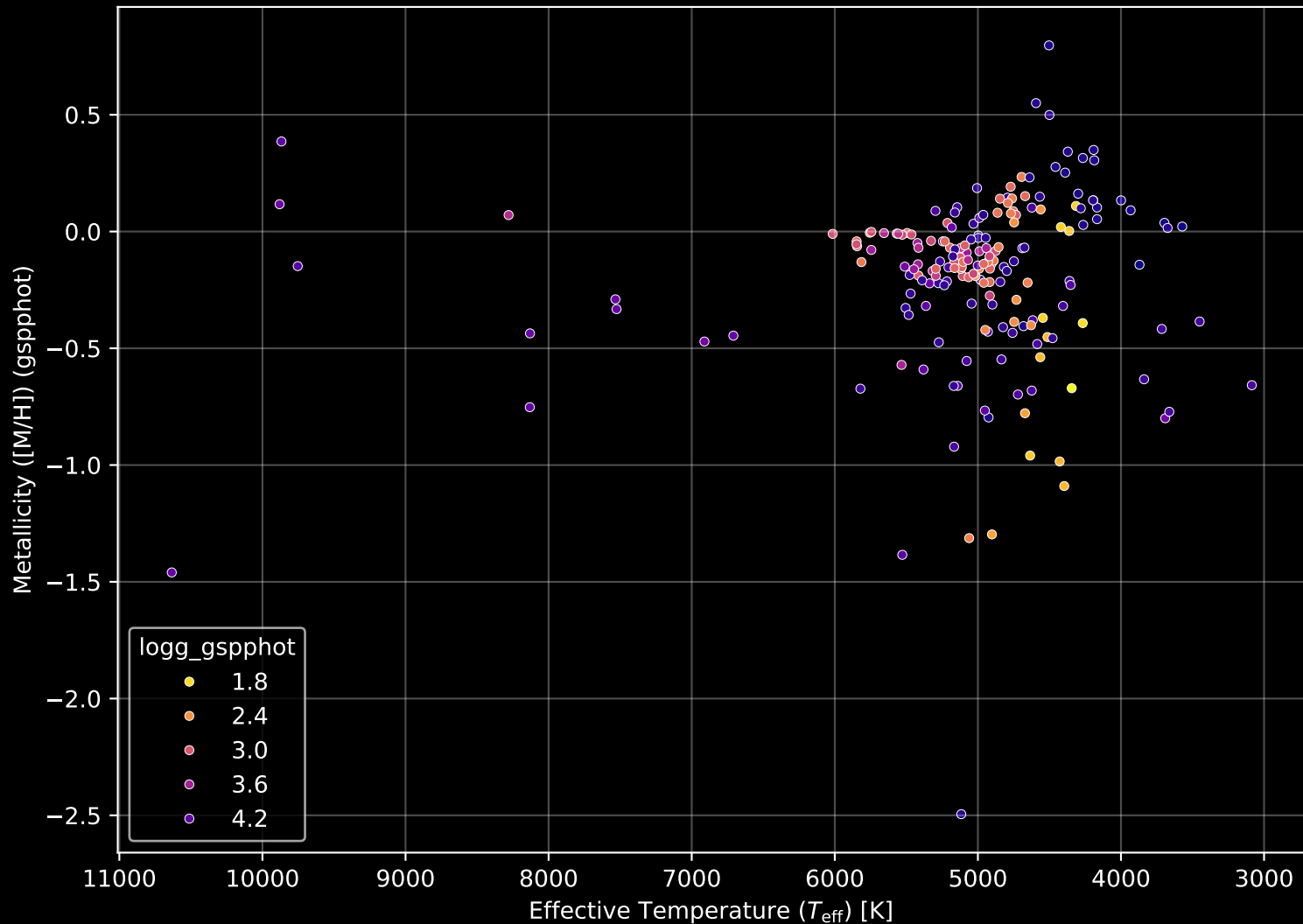
APOGEE DR17 Field: [K2_C4_168-21_btx] Stellar Population Parameters (n= 193)
